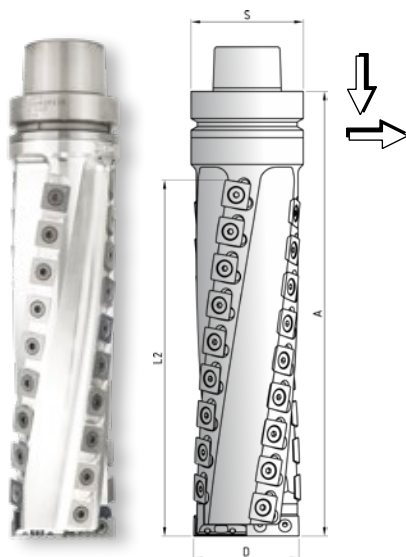
HW Spiralfräser Z=2R/R TC Helicoidal cutter Z=2R/R
