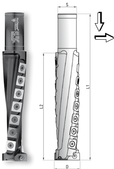
HW Spiralfräser Z=2R/R TC Helicoidal cutter Z=2R/R
