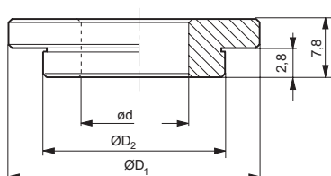
Stahl-Reduzierring Steel-reducing sleeve
