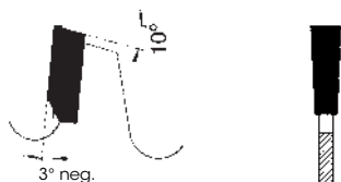
Flachzahn, negativer Spanwinkel Flat tooth, negative chip angle
