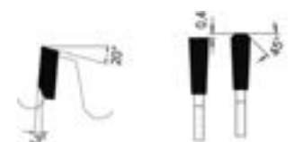
Trapez-Flachzahn negativer Spanwinkel Trapezoidal flat tooth with neg. rake angle
