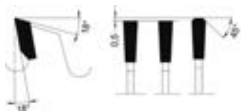
Flach-Flach-Trapezzahn Flat-Flat-Triplechip
