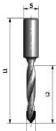
Type 1: Z=2
