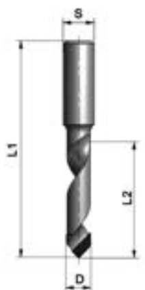
Type 1: Z=1
