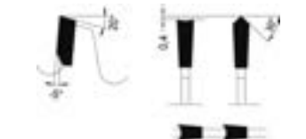
Hohlzahn-Dach-Flach neg. Spanwinkel Hollow tooth/inverted V/flat tooth, neg. rake angle
