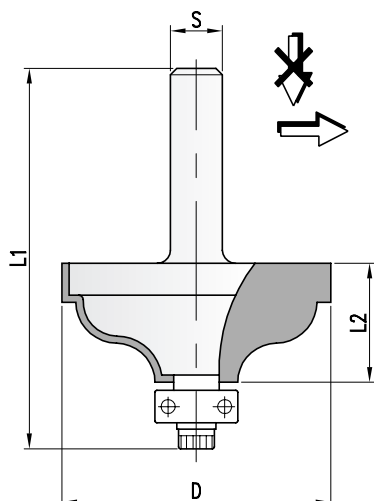
HW Profilfräser Z=2 TC Profilecutter Z=2
