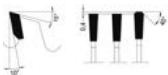
Trapez-Flach-Flachzahn Triple-Flat-Flattooth
