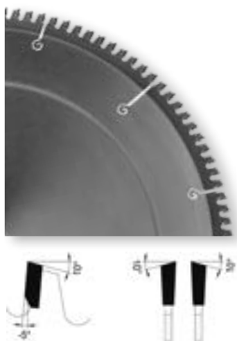
Wechselzahn neg. Spanwinkel Alternate top bevel tooth with neg. rake angle
