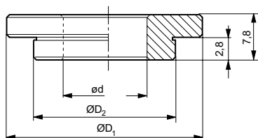
Stahl-Reduzierring Steel-reducing sleeve
