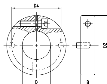
Klemmring Locking ring
