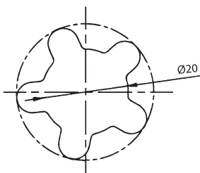
Festool FastFix Bohrbild Festool FastFix pattern drawing
