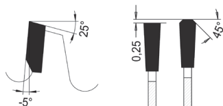
Trapez-Flachzahn, negativ Triple Chip Grind tooth, negative
