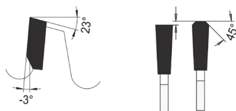
Trapez-Flachzahn, negativer Spanwinkel Trapezoidal Flat Tooth, negative rake angle
