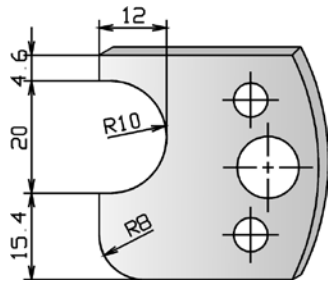
Art.Nr. Profilmesser - profile knives 778.104 Abweiser - limiters 778.204
