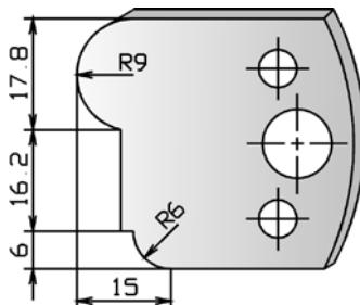
Art.Nr. Profilmesser - profile knives 778.155 Abweiser - limiters 778.255
