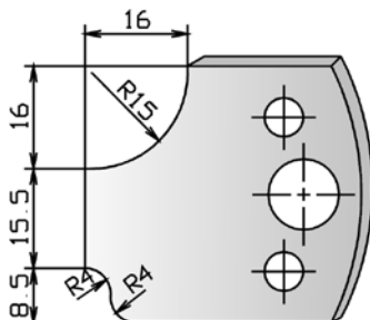
Art.Nr. Profilmesser - profile knives 778.143 Abweiser - limiters 778.243
