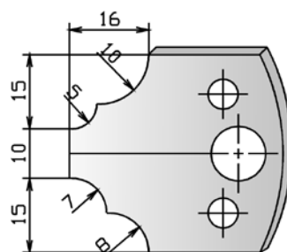
Art.Nr. Profilmesser - profile knives 778.122 Abweiser - limiters 778.222
