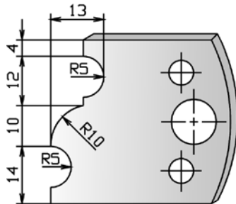
Art.Nr. Profilmesser - profile knives 778.152 Abweiser - limiters 778.252
