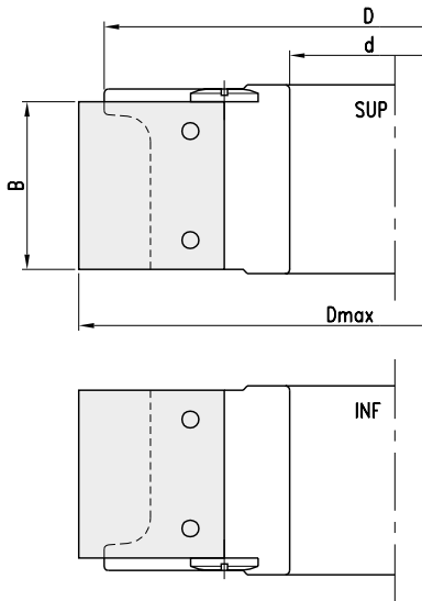
Typ E: Standardblankett type E: standard blank knife
