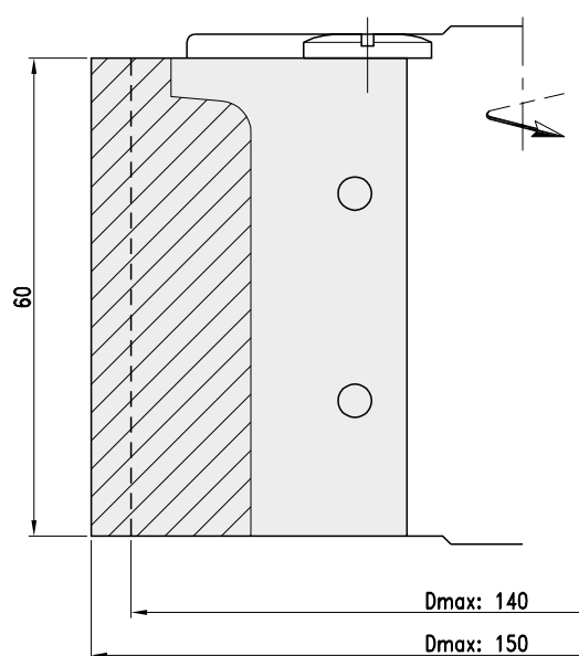
Standardblankett standard blank knife
