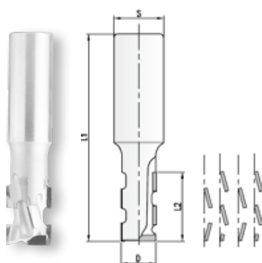
PKD-Schaftfräser ECO PCD shank milling cutter ECO
