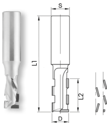
PKD-Schaftfräser ECO PCD shank milling cutter ECO
