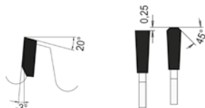
Trapez-Flachzahn, negativer Spanwinkel Triple Chip Grind tooth with negative rake angle
